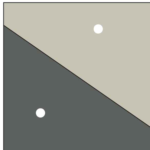
Split the plane along this line
