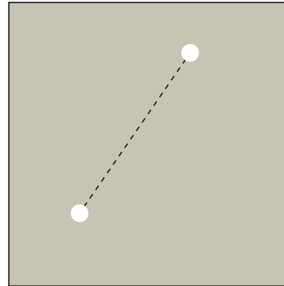
Draw a second dot anywhere and draw a line connecting the dots' centers
