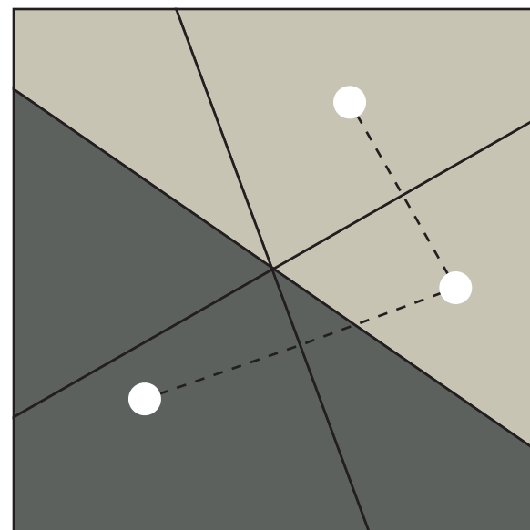
Draw a new point anywhere on the plane; the process is repeated, though a line is now drawn between the existing two points and extended to the edges
