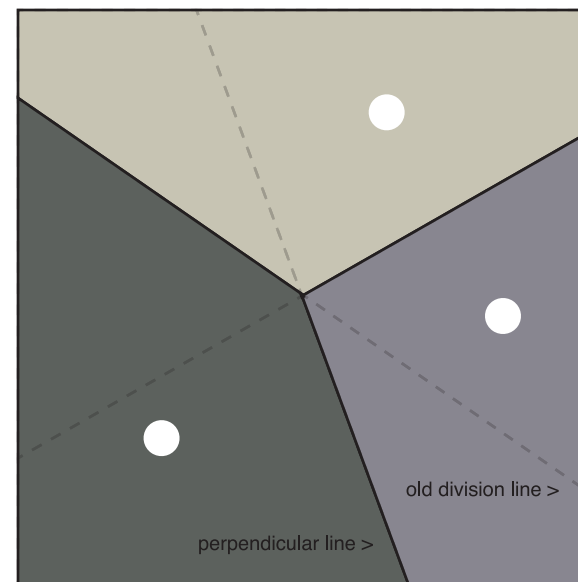
The plane is one again split - the plane containing the dot is retained, as are any neighbors between the dot and the newest perpendicular lines
