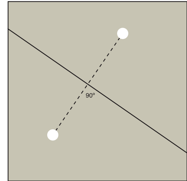
At the midpoint of the line between the two points, draw a line that is perpendicular and extend to the edges of the plane
